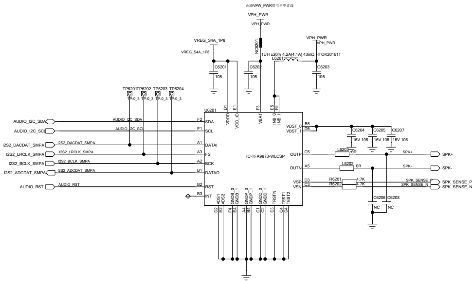
TFA9873 I2C Address (R:0x69; W:0x68)
